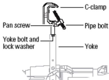
Mounting section of a lighting instrument
