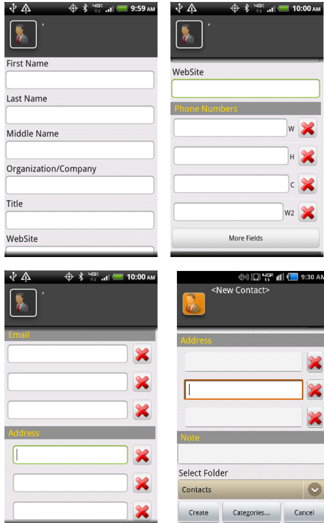
FIGURE 15. New Contact Screen
