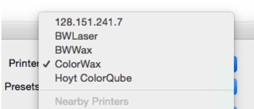
Figure 13. New Printers
