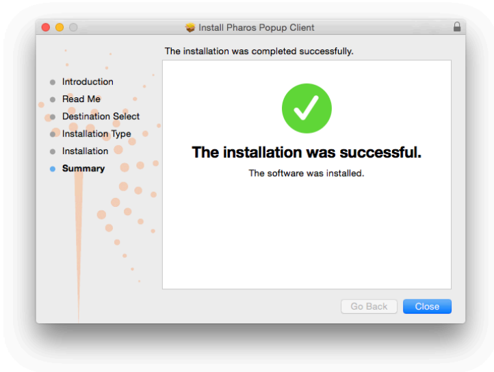
Figure 12. Installation Success
