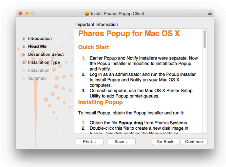
Figure 9 Quick Start
