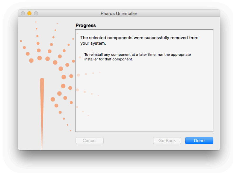
Figure 5. Uninstallation Success
