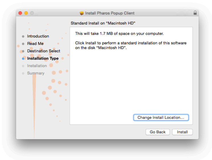
Figure 10 Confirmation
