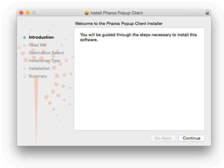
Figure 8 Installer
