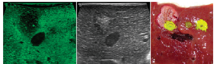
Figure 1. Sonoelastography image of a RFA lesion in vivo (left). Corresponding B-mode image of the lesion (center). Gross pathology of the lesion (right).
